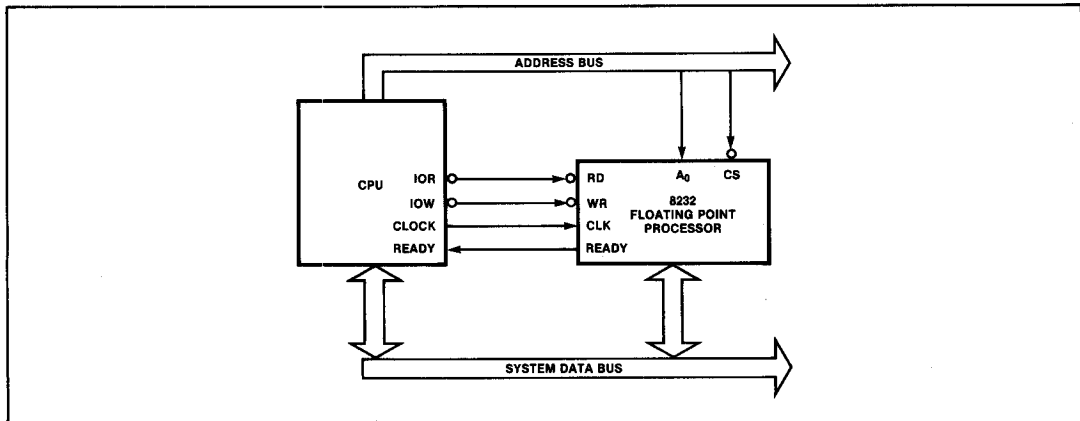
Figure 3. Minimum Configuration Example
