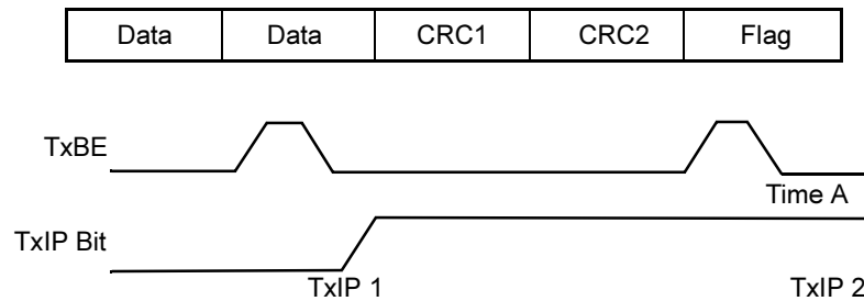
Figure 14. TxIP Latching
