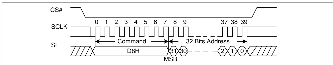
Figure 48 64KB Block Erase with 4-Byte Address Sequence Diagram (ADS=0 or ADS=1)
