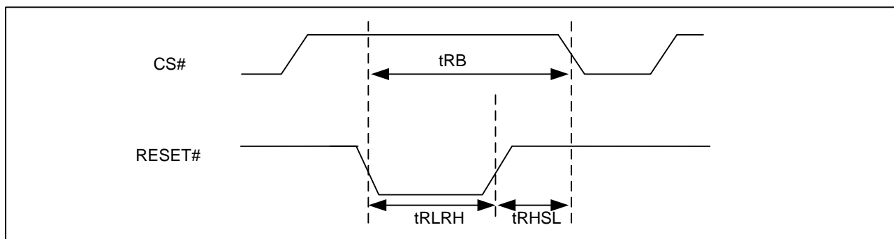
Figure 77 RESET Timing
