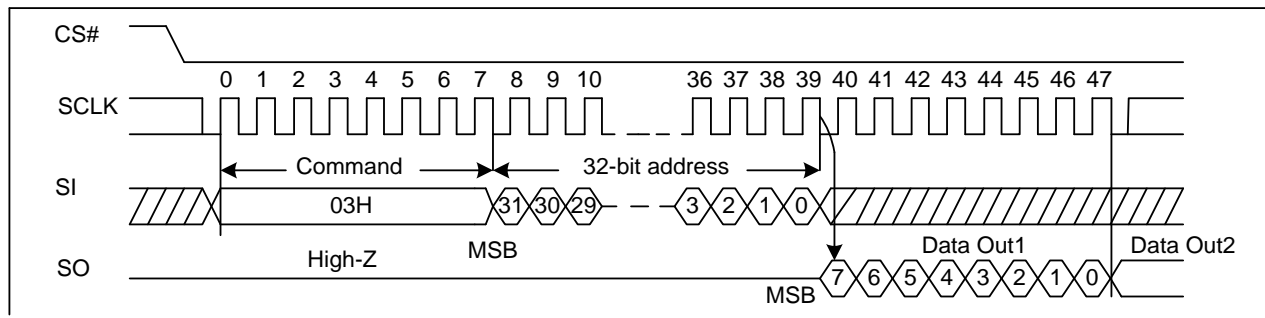
Figure 10 Read Data Bytes Sequence Diagram (ADS=1)
