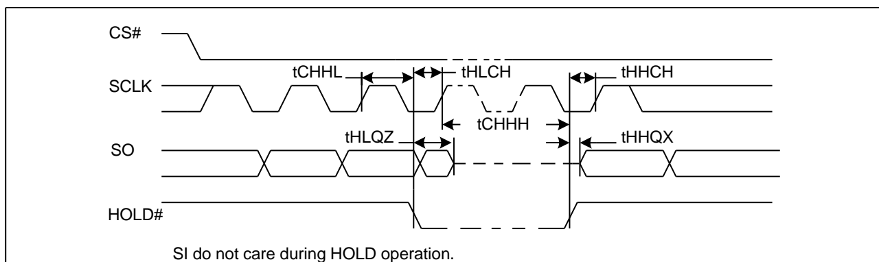
Figure 76 Hold Timing
