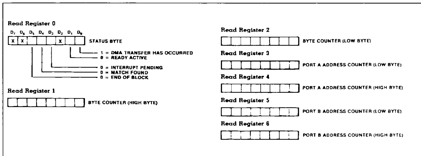
Figure 8a : Read Registers.
