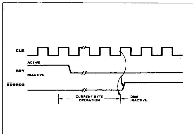
Figure 18 : Bus Release When Not Ready (Burst Mode).
