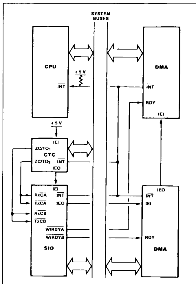
Figure 3 : Typical Z80 Environment.
