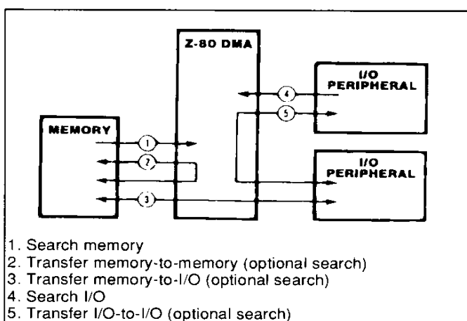
Figure 4 : Function of the Z80 DMA.
