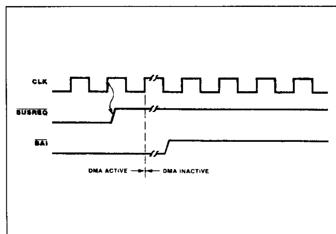
Figure 16 : Bus Release (Byte-at-a-Time-Mode).
