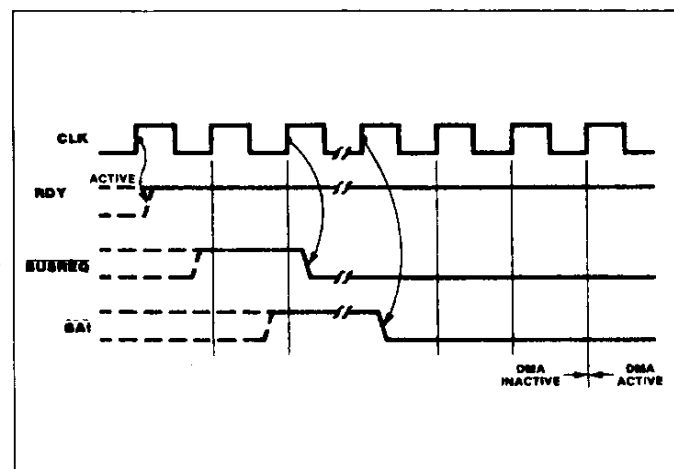
Figure 15 : Bus Request and Acceptance.
