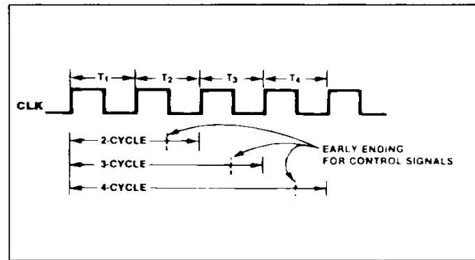
Figure 5 : Variable Cycle Length..
