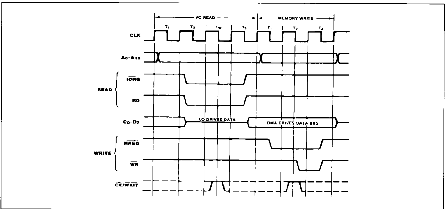
Figure 13 : I/O-to-Memory Transfer.
