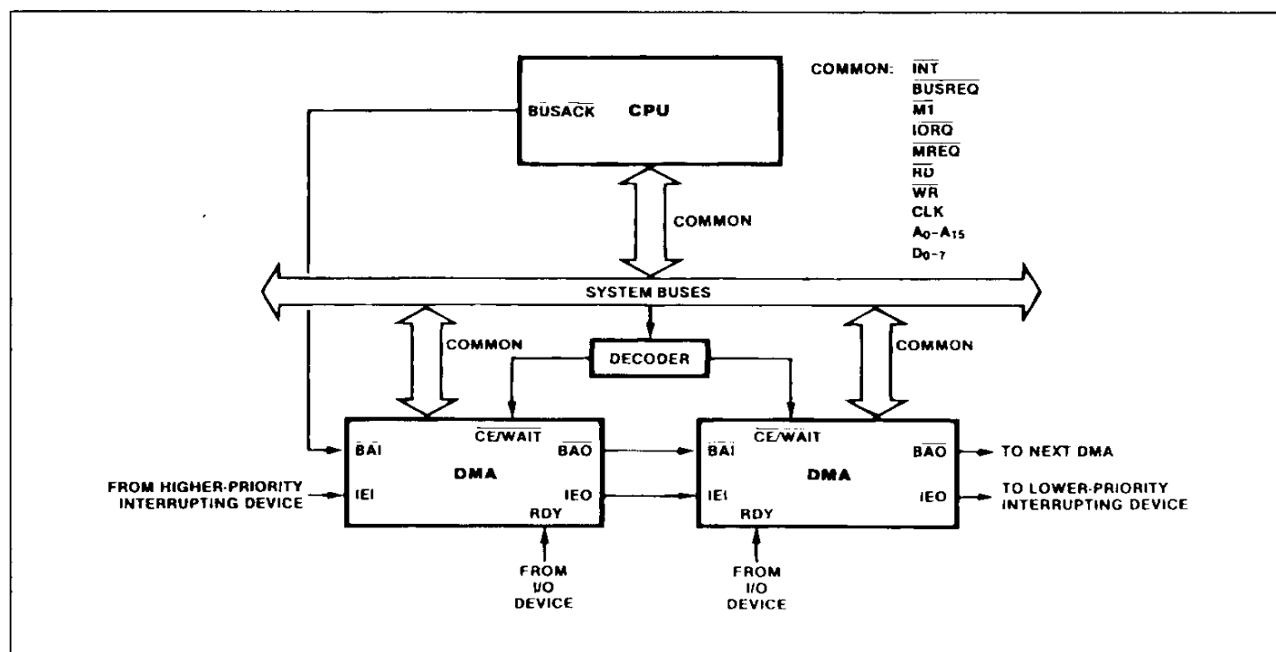
Figure 7 : Multiple-DMA Interconnection to the Z80 CPU.
