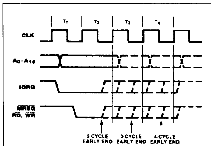
Figure 14 : Variable-Cycle and Edge Timing.
