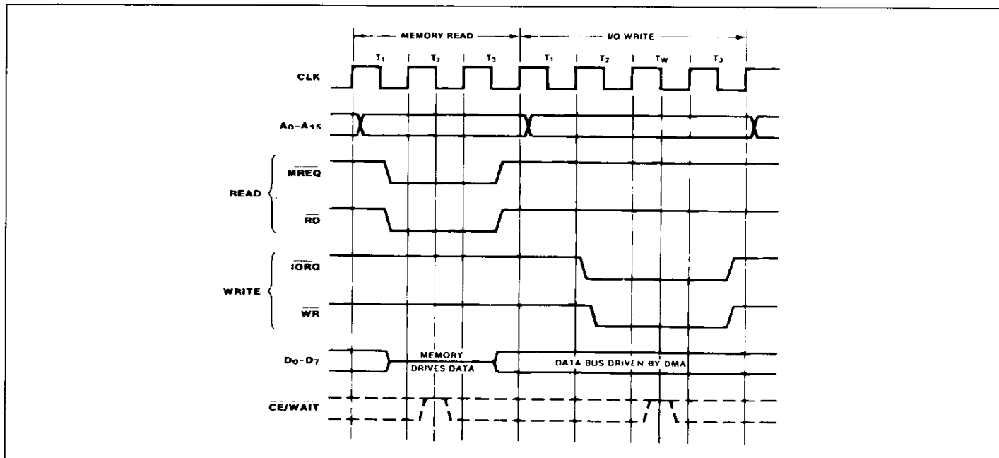
Figure 12 : Memory-to-I/O Transfer.
